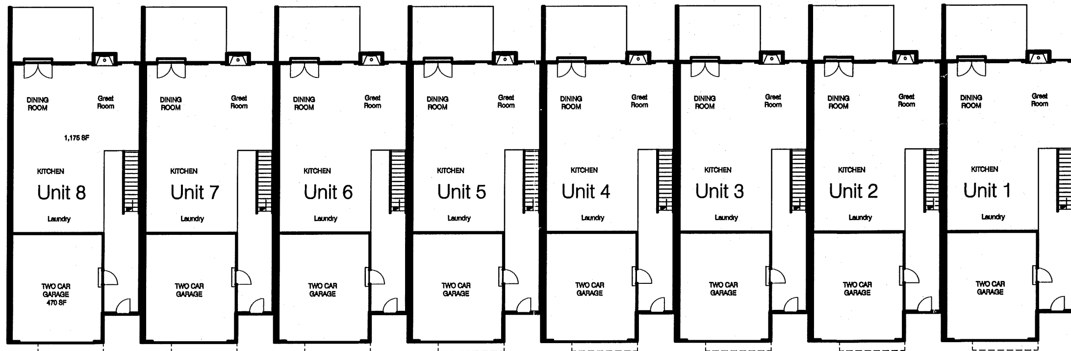
STREET LEVEL PLAN
