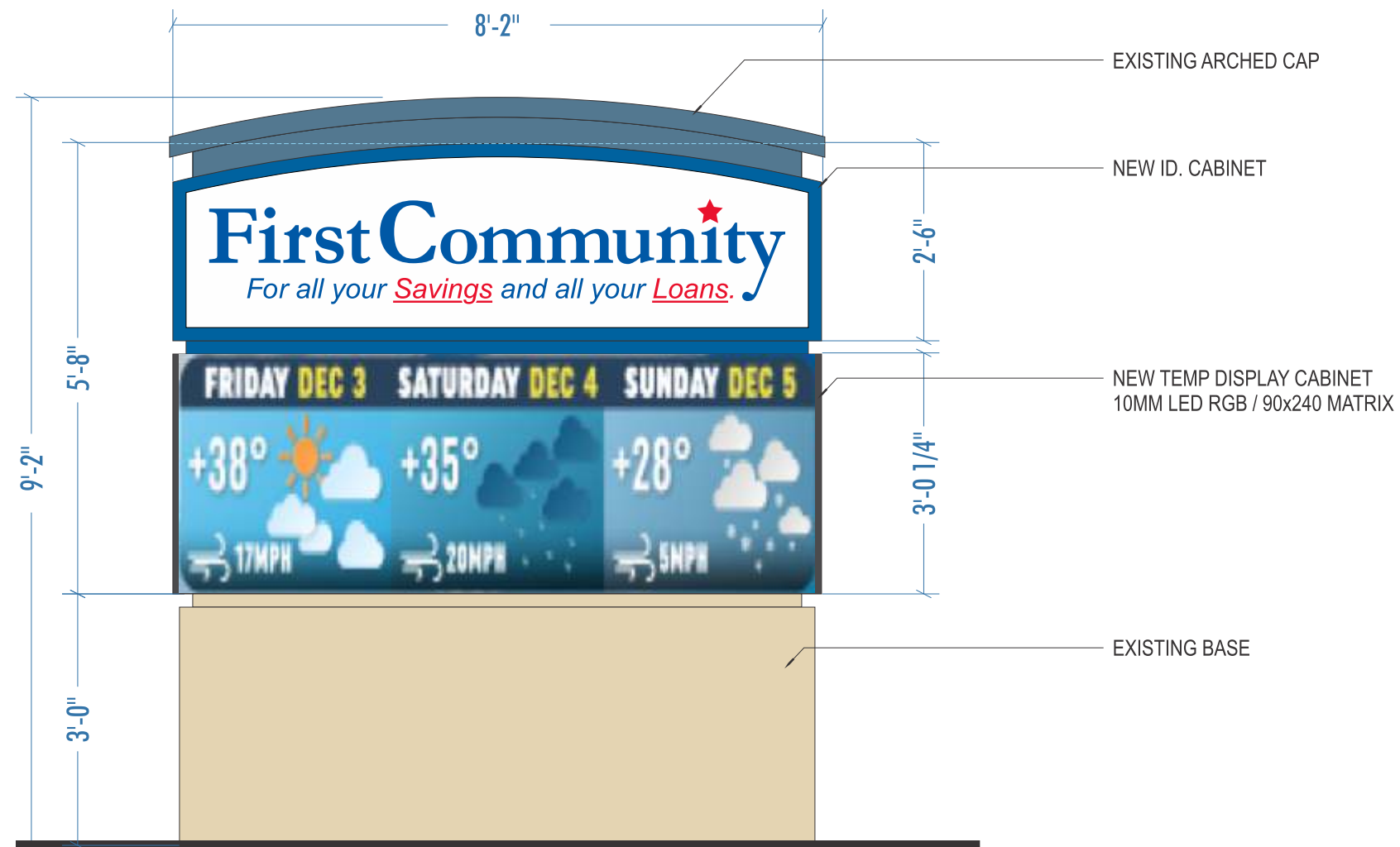
FRONT ELEV (D/F SIGN)
