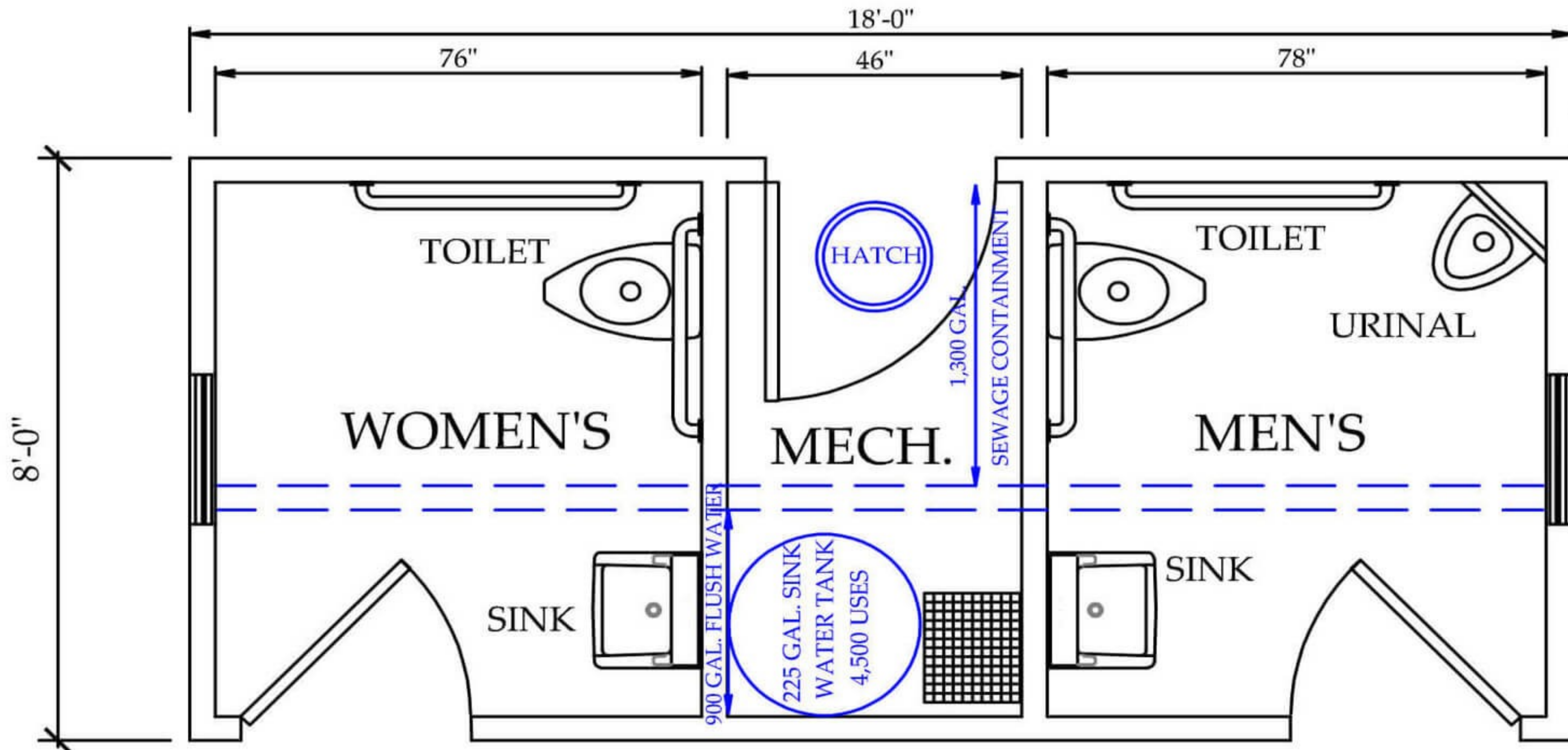
MALE / FEMALE FLOOR PLAN DOUBLE UNISEX PLAN SIMILAR
